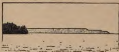
FIG. 368. — The notched rock headland of Boyer Bluff between Green Bay and Lake Michigan (after Goldthwait).
